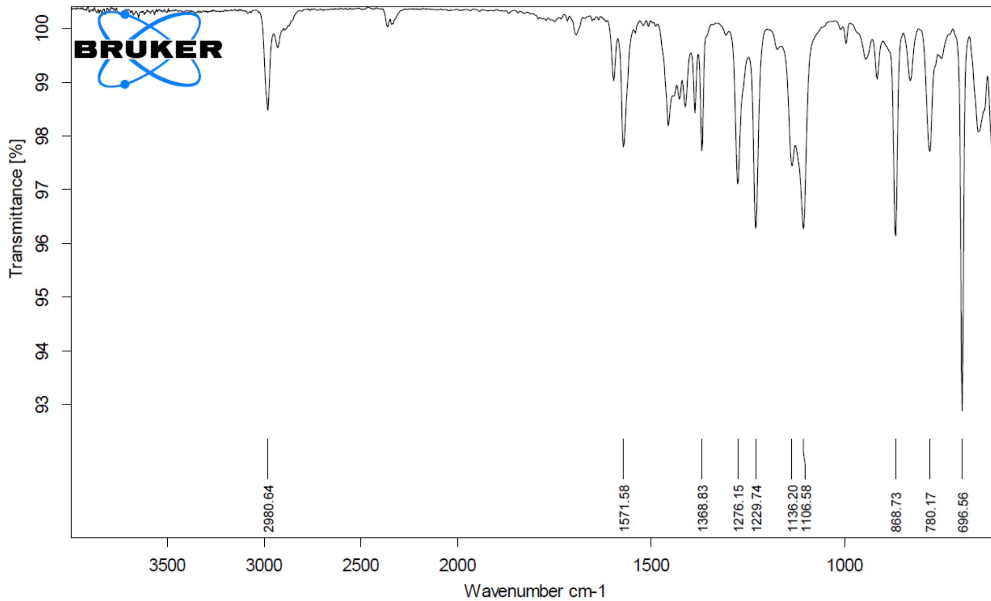
IR of 1-bromo-3,5-bis(1-chloro-1-methylethyl)benzene ( 3 )
